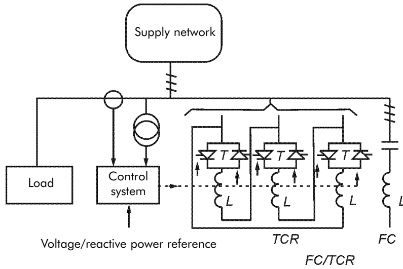
Figure 12 - Three phase FC/TCR compensator
