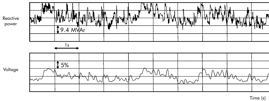
Figure 4 - Changes in the reactive power and the resulting voltage fluctuations at the point of connection of an arc furnace
