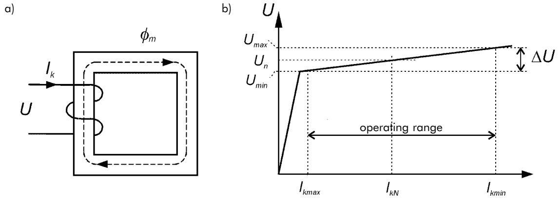
Figure 9 - Principle of operation of the self-saturable reactor: schematic diagram (a), magnetic characteristic of the core (b)
