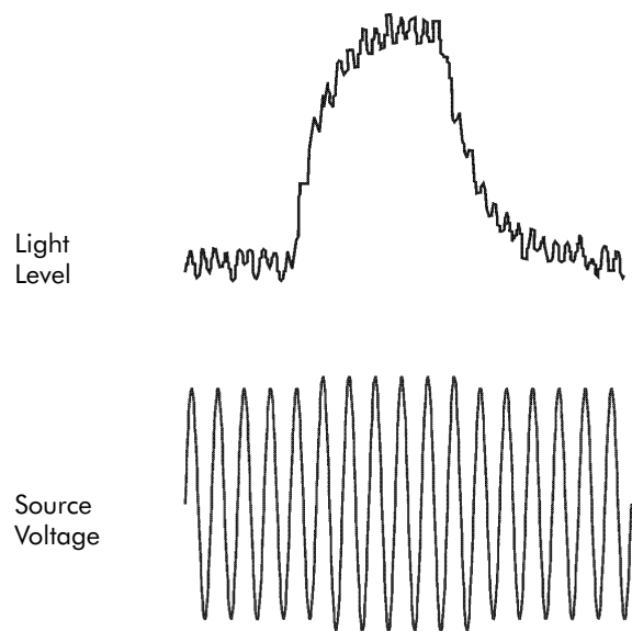
Figure 6 - The effect of a voltage change on the luminous flux of an incandescent lamp [1]
