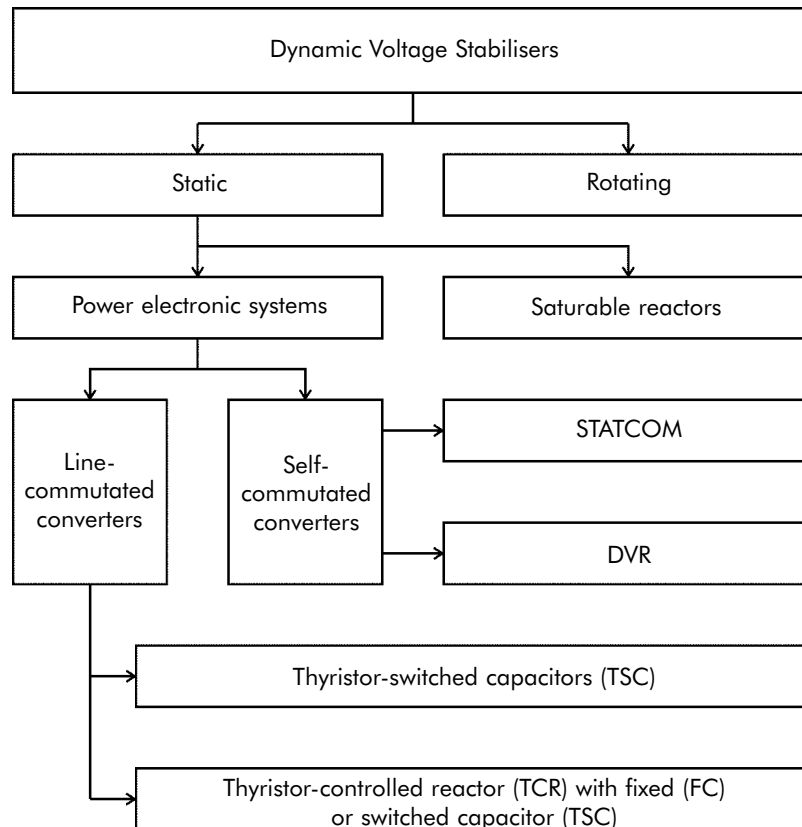
Figure 7 - Classification of dynamic voltage stabilisers
