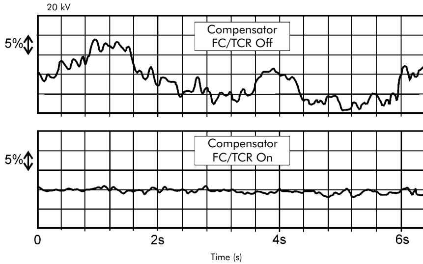
Figure 13 - An example effect of compensator FC/TCR performance
