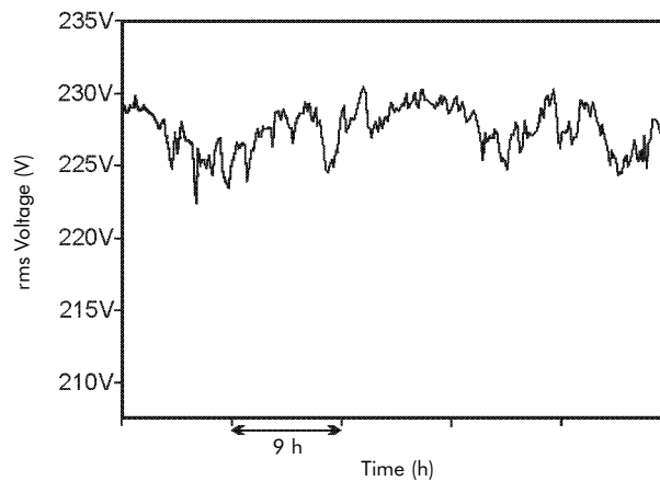
Figure 3 - Example of rms voltage fluctuation
