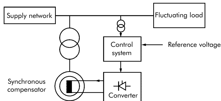
Figure 8 - Voltage stabilisation control system using a synchronous compensator
