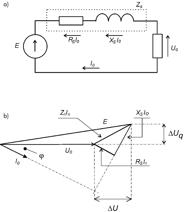
Figure 2 - Per-phase equivalent circuit of supply network (a) and phasor diagram for a resistive-inductive load E \geq U_0 (b)
