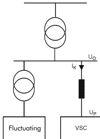
Figure 14 - Schematic diagram of a compensator (VSC) connected to the supply network
