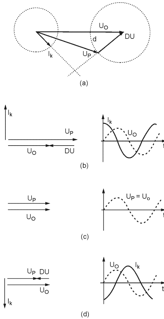
Figure 15 - STATCOM voltage and current waveforms and phasor diagrams for different phase relationships between U_0 and U_P
