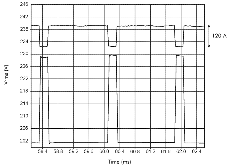
Figure 5 - Power system voltage fluctuation during welding work
