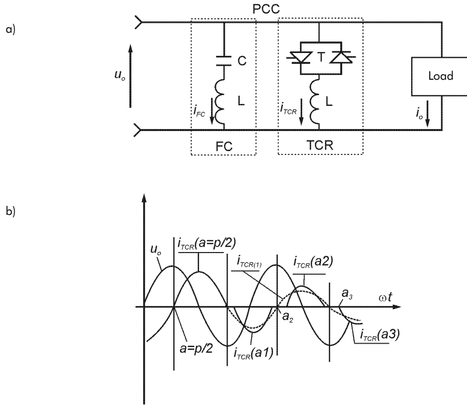
Figure 11 - Conceptual diagram of a single-phase FC/TCR compensator (a), TCR current waveforms (b)
