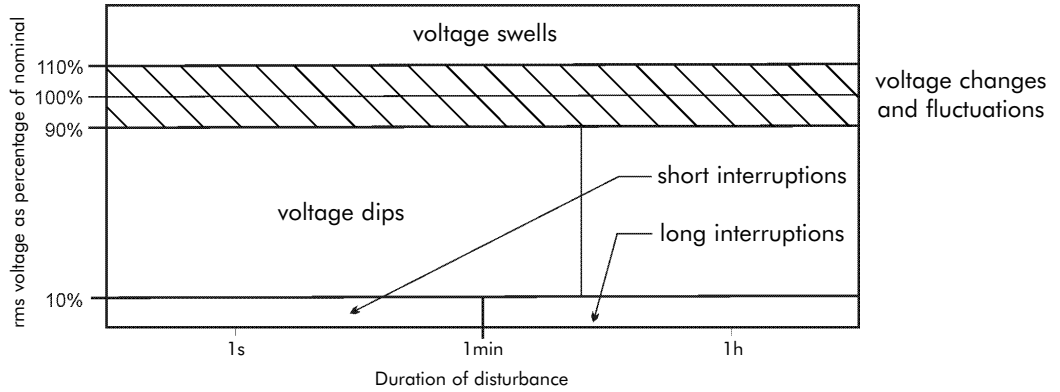
Figure 1 - Classification of voltage variations
